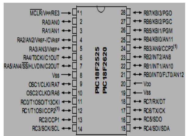
Figure 3: PIN layout of PIC18F2620 [21]
